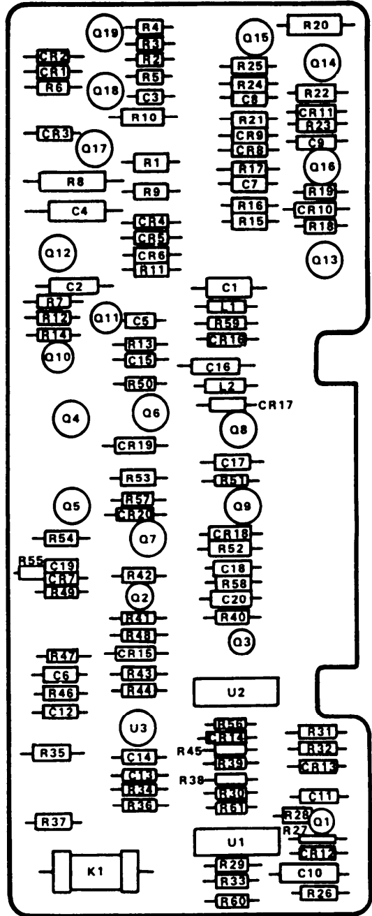
Figure 9. Circuit Card Assembly, Deflection Amplifier
