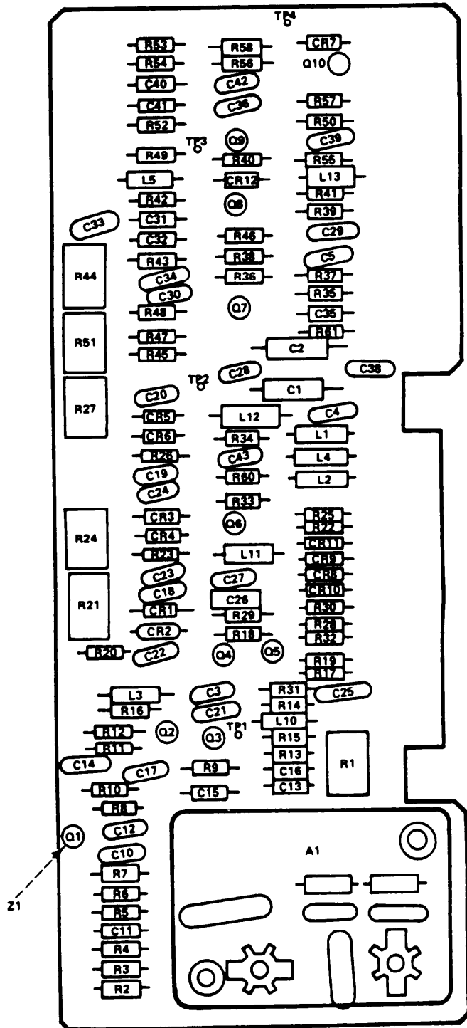
Figure 3. 3-MHz Amplifier Board Assembly
