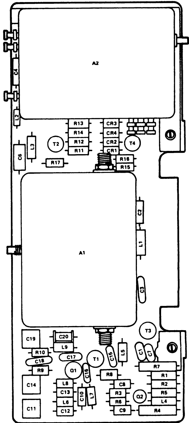
Figure 5. 50-MHz Converter
